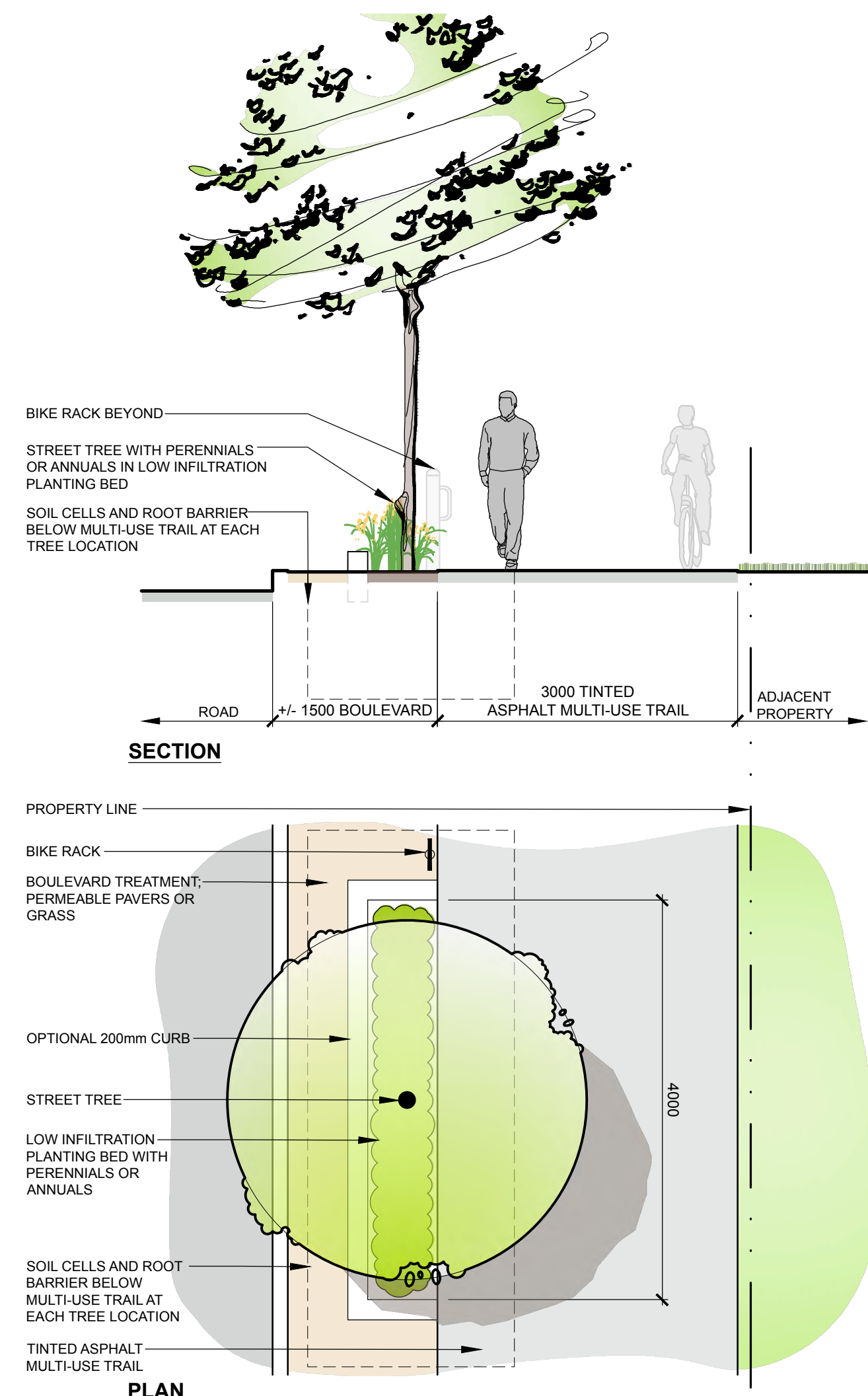
1 TYPICAL MULTI-USE TRAIL LAYOUT L3 N.T.S.
